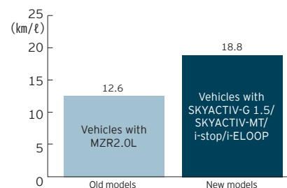
j Comparison of Fuel Economy between New and Old Models (Roadster(MX-5 overseas), fuel economy at Japanese JC08 mode test cycle)
