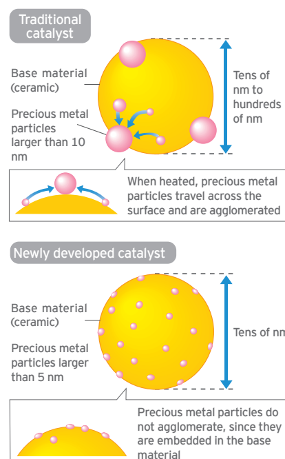
p Model of precious metal dispersion by new catalyst technology
